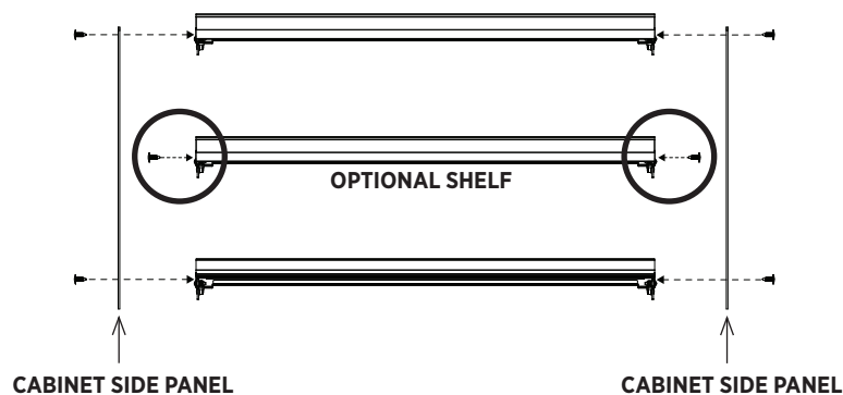
DETAIL 24B DIAGRAM SHOWING INSTALLATION OF A SINGLE STORAGE CABINET
